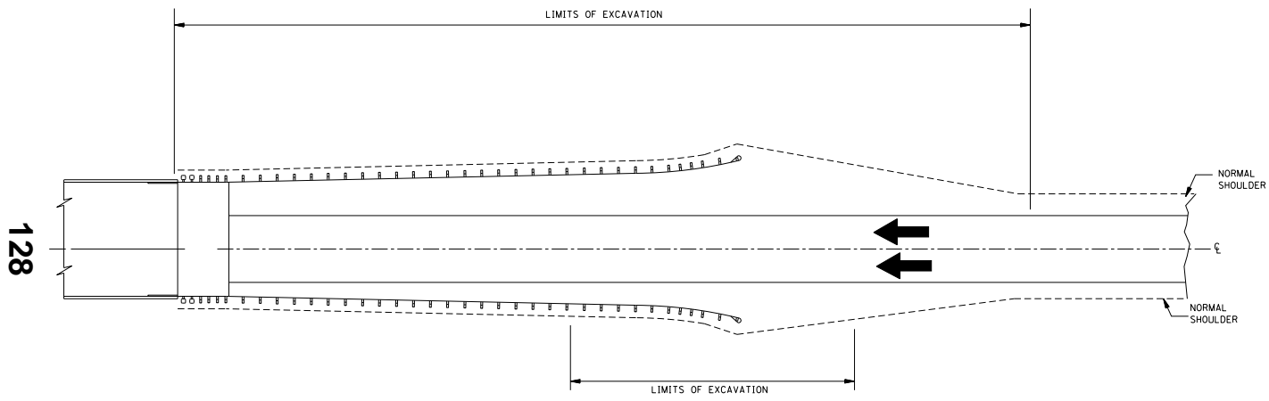
DIVIDED HIGHWAY WITH BARRIER OUTSIDE CLEAR ZONE OF OPPOSING TRAFFIC
