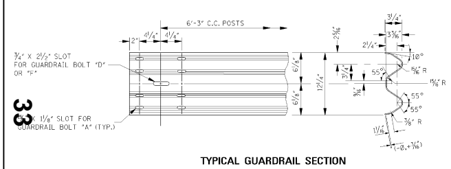
TYPICAL GUARDRAIL SECTION
