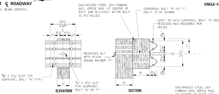
GUARDRAIL SPLICE DETAIL
