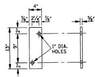
DETAIL OF PLATE "B"
