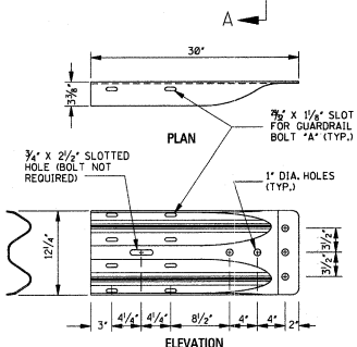
"W" BEAM TERMINAL CONNECTOR
