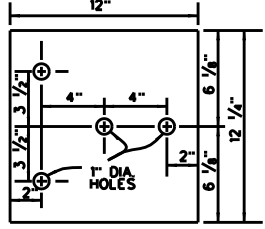
DETAIL OF BACK PLATE
