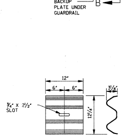
"W" BEAM BACKUP PLATE
