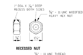
HEX NUT AND BOLT "F"
