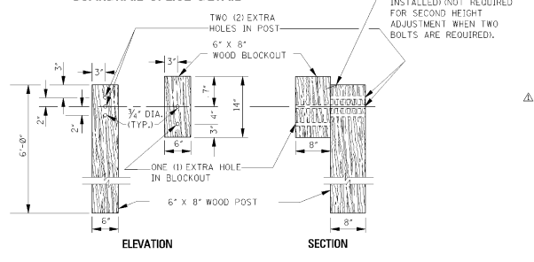
DETAILS OF ADJUSTABLE HEIGHT BLOCKOUT ASSEMBLY
