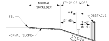
SECTION D-D FOR OBSTACLES 17' OR MORE FROM NORMAL SHOULDER
