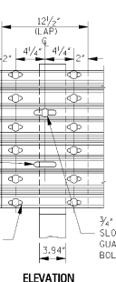
GUARDRAIL SPLICE DETAIL
