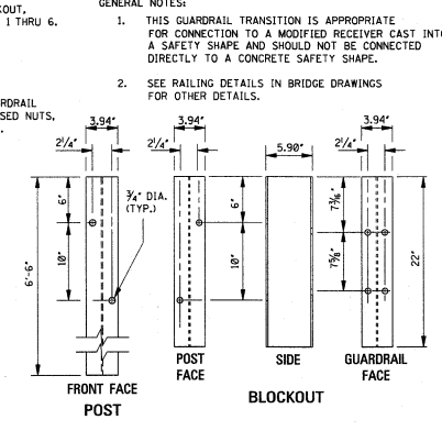
DETAILS OF THRIE-BEAM POST AND BLOCKOUT (POST 1 THRU POST 6)
