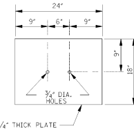
SOIL PLATE NOTE: 2 REQUIRED
