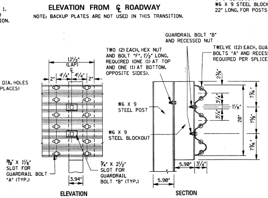
GUARDRAIL SPLICE DETAIL (POST 5)
