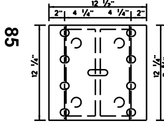
FRONT ELEVATION SHOWING 10 GA. GUARD RAIL CONNECTION TO W12x50 BACK OF RAIL PLATE & BACK OF BRACKET
