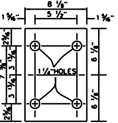
FRONT ELEVATION SHOWING 10 GA. GUARD RAIL CONNECTION TO W12x50 BACK OF RAIL PLATE & BACK OF BRACKET
