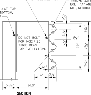
GUARDRAIL SPLICE DETAIL
