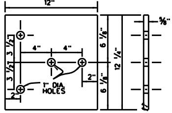
DETAIL OF FRONT PLATE
