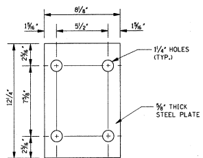
DETAIL OF PLATE "B"
