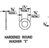
FASTENER DETAILS
