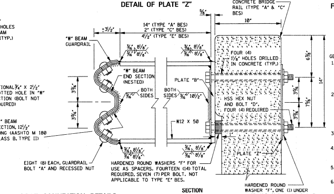
GUARDRAIL CONNECTION DETAILS
