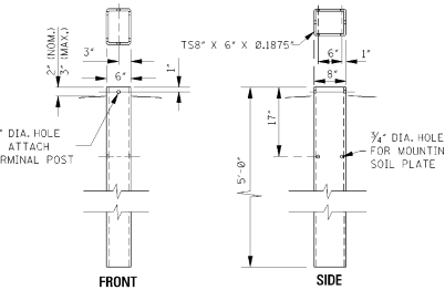
STEEL TUBE ANCHOR
