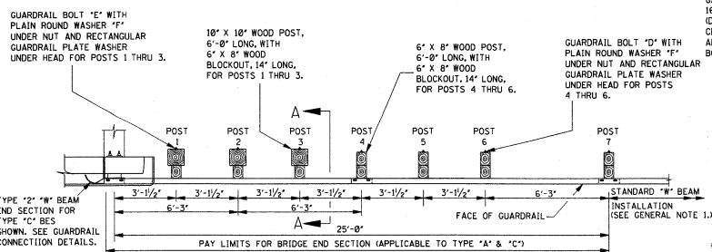
PLAN OF BRIDGE END SECTION
