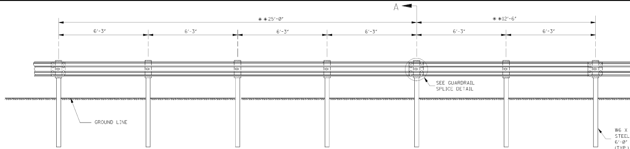
ELEVATION FROM \zeta ROADWAY ** NOTE: OPTIONAL BEAM LENGTHS.
