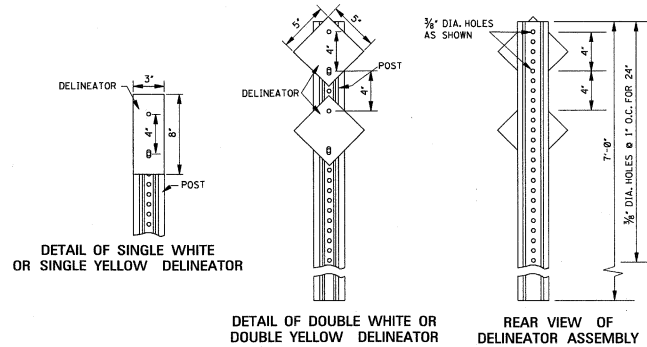
DETAIL OF SINGLE WHITE OR SINGLE YELLOW DELINEATOR DETAIL OF DOUBLE WHITE OR DOUBLE YELLOW DELINEATOR REAR VIEW OF DELINEATOR ASSEMBLY MOUNTING DETAIL DELINEATORS, OBJECT MARKERS OR DISTANCE REFERENCE SIGNS (D10-1, D10-2, OR D10-3) ARE MOUNTED TO THIS FACE AS SHOWN. DIRECTION OF TRAFFIC
