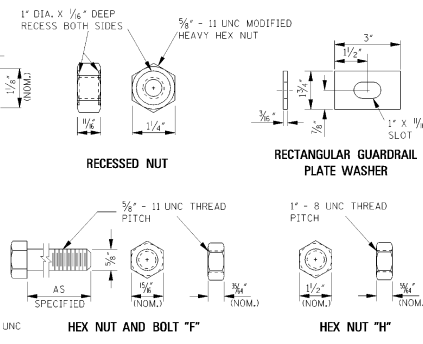
FASTENER DETAILS
