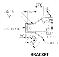
ANCHOR PLATE ASSEMBLY DETAILS
