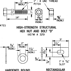
FASTENER DETAILS
