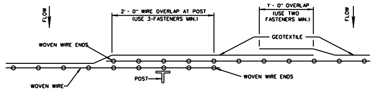
PLAN VIEW REQUIRED LAPPING
