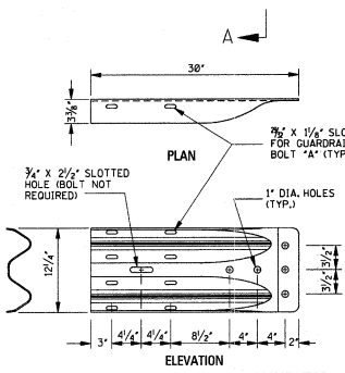
"W" BEAM TERMINAL CONNECTOR NOTE: THE "W" BEAM TERMINAL CONNECTOR IS USED WITH THE TYPE "H" BRIDGE END SECTION. THE CROSS-SECTIONAL DIMENSIONS OF THIS PART ARE IDENTICAL TO THE STANDARD "W" BEAM SECTION (AASHTO M 180 CLASS B, TYPE III).
