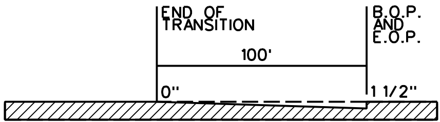
MILLING TRANSITION AT B.O.P. AND E.O.P.
