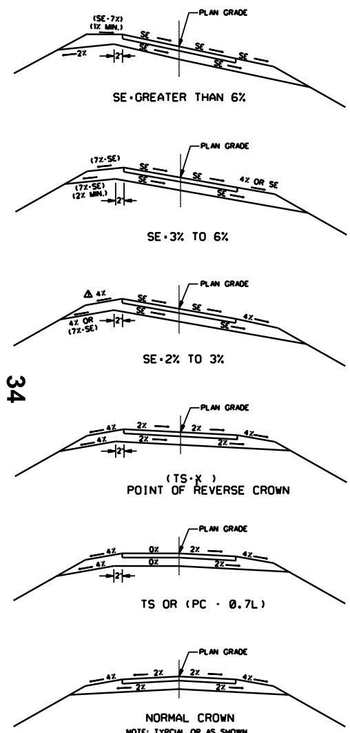
DETAILS OF SHOULDER & SUBGRADE TREATMENT
