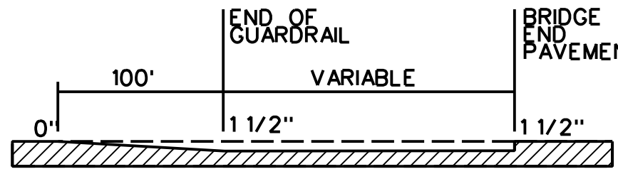
MILLING TRANSITION AT BRIDGE END PAVEMENT
