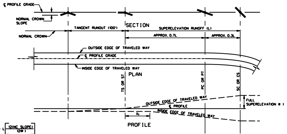
DIAGRAMMATIC PLAN AND PROFILE
