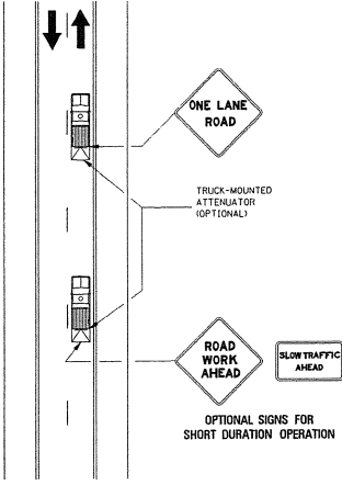
MOBILE OPERATIONS ON TWO-LANE ROAD
