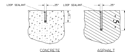
DETAIL OF CABLE SLOT NOT TO SCALE
