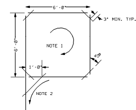
1. INSTALL WIRE TURNS THE SAME (CLOCKWISE) DIRECTION. 2. LOOP LEAD WIRE EXIT FROM LAST TURN 3. ALL LOOPS TO INCLUDE 4 TURNS OF #14WG WIRE. 4. DIMENSIONAL TOLERANCE FOR LOOP LENGTH, SPACING AND DETECTOR LOCATION: 1 /2'.
