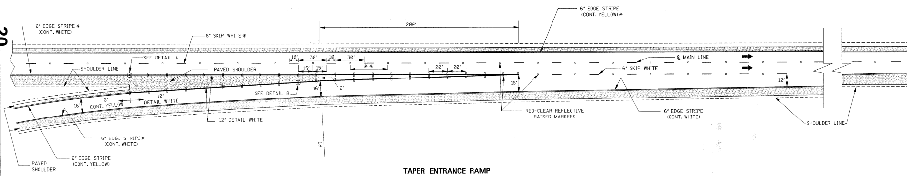
TAPER ENTRANCE RAMP
