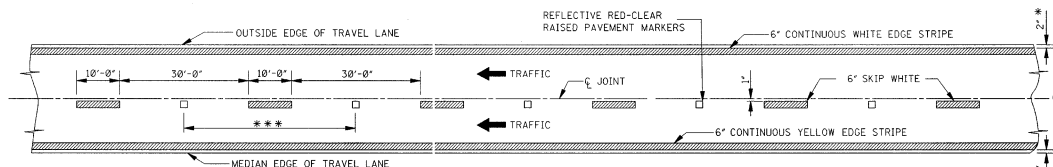
4-LANE: WITH ONE-WAY TRAFFIC
