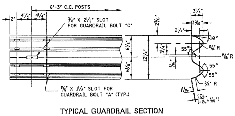
TYPICAL GUARDRAIL SECTION
