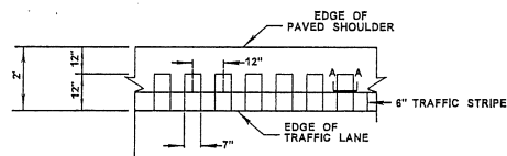
DETAIL "A"
