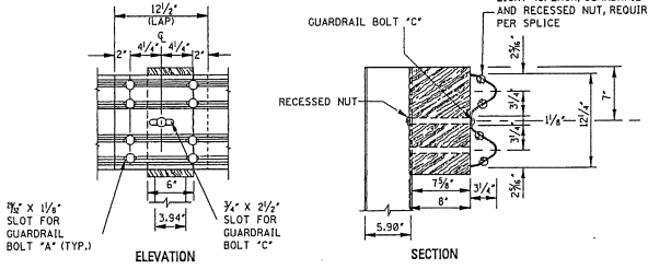
GUARDRAIL SPLICE DETAIL
