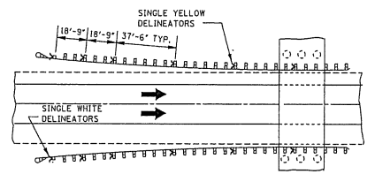
ROADSIDE OBSTACLE INSTALLATION—LENGTH 250' OR LESS (ONE-WAY TRAFFIC)
