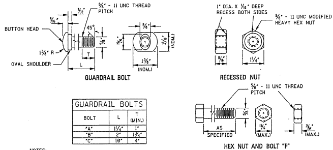
FASTENER DETAILS
