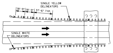
ROADSIDE OBSTACLE INSTALLATION—LENGTH 250' OR LESS (ONE-WAY TRAFFIC)
