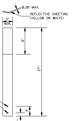
DETAIL OF FLEXIBLE GUARDRAIL DELINEATOR
