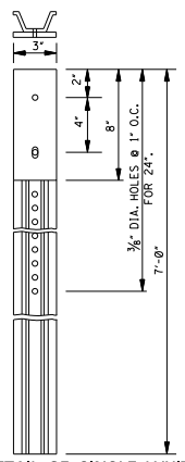
DETAIL OF SINGLE WHITE OR SINGLE YELLOW DELINEATOR
