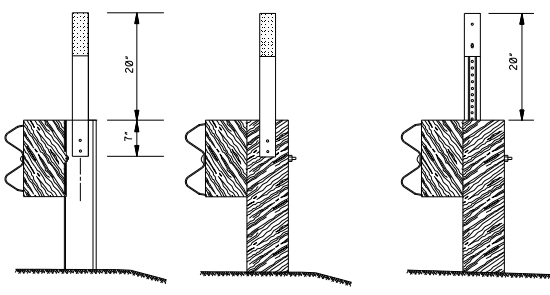
TYPICAL FLEXIBLE POST DELINEATOR GUARDRAIL INSTALLATION
