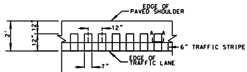
DETAIL "A"
