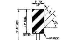
VERTICAL PANEL
