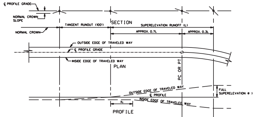
DIAGRAMMATIC PLAN AND PROFILE
