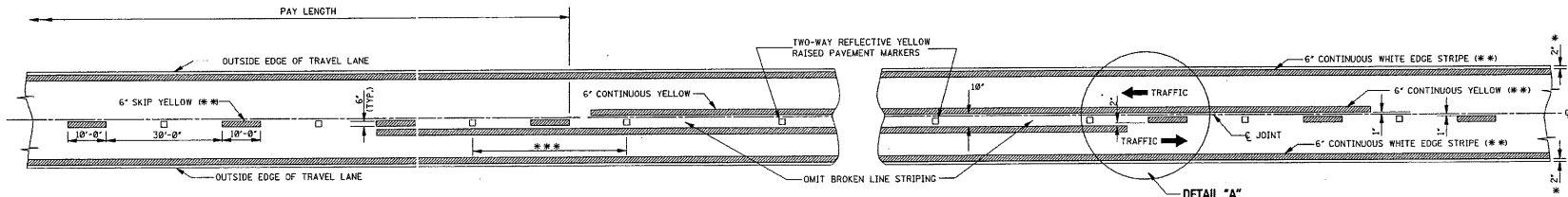
TWO-WAY TRAFFIC (ASPHALT OR CONCRETE PAVEMENT)
