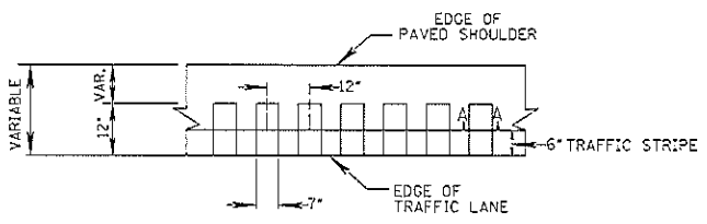
DETAIL "A"
