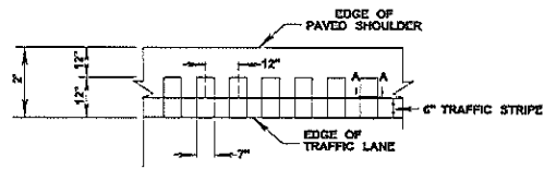
DETAIL "A"
