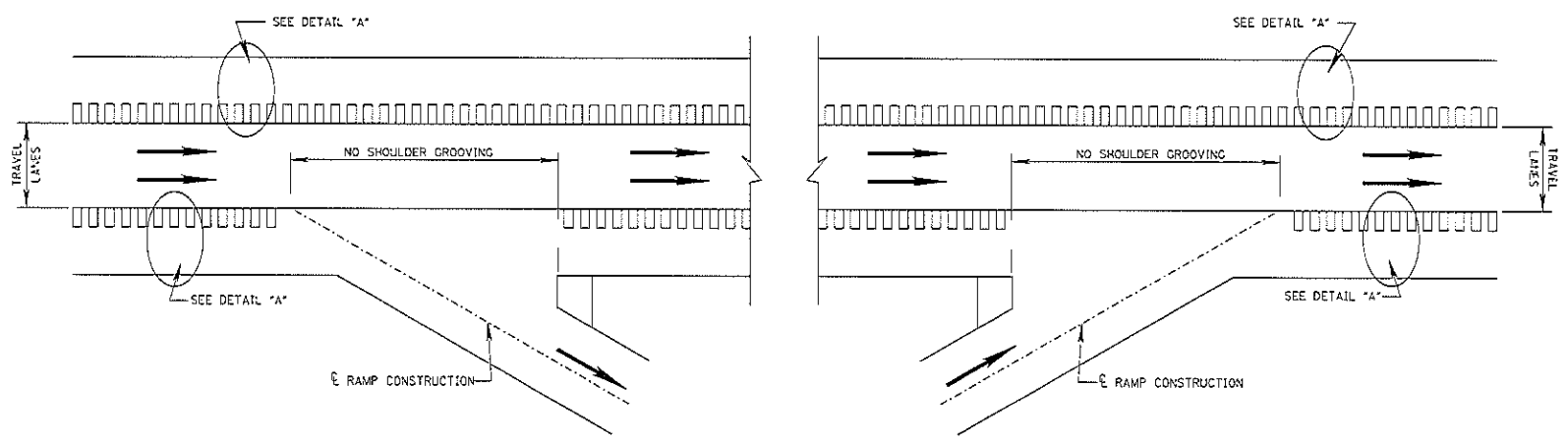
PLAN NOT TO SCALE DETAILS OF RUMBLE STRIPS (GROUND-IN)
