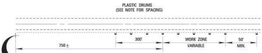
TYPICAL SHOULDER WORK #2
