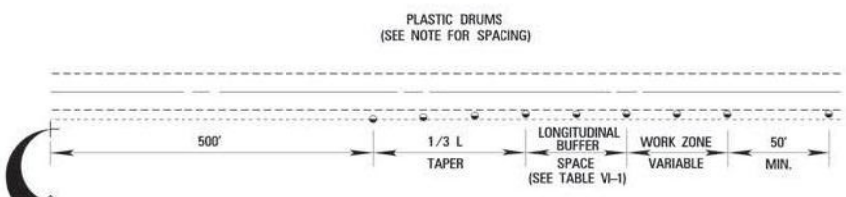
TYPICAL SHOULDER CLOSURE
