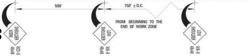
TYPICAL SHOULDER WORK #1
