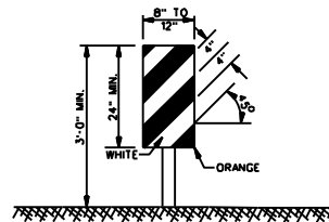
VERTICAL PANEL
