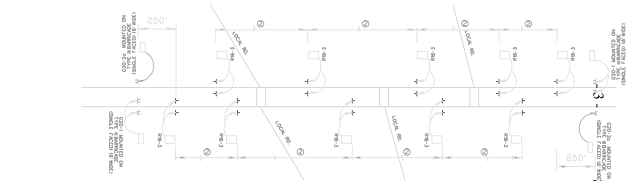
DIVIDED HIGHWAY SHOWN (2 LANE - 2 WAY ROADWAY SIMILAR) (PROJECT MORE THAN 1 MILE LENGTH)
