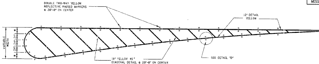
DETAIL A * NOTE: VARIABLE (24" MAXIMUM)
