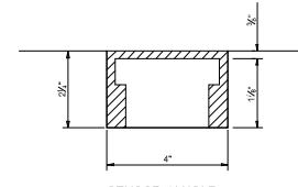
SENSOR IN HOLE WITH EPOXY
