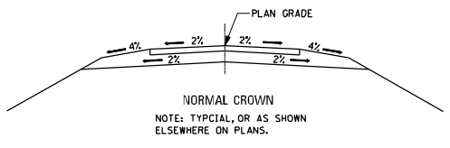
DETAILS OF SHOULDER & SUBGRADE TREATMENT
