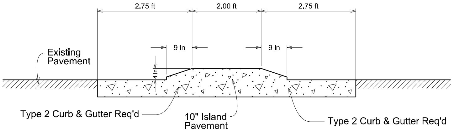
Typical Section
