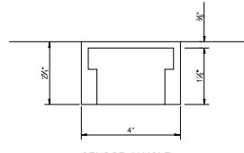
SENSOR IN HOLE SIDE VIEW
