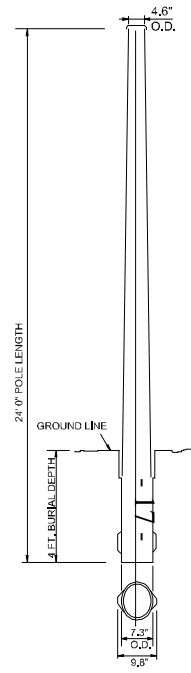
REPEATER POLE ASSEMBLY
