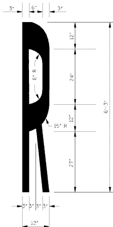
DETAIL A STANDARD "R" PAVEMENT MARKING FOR X R X R SYMBOL
