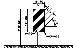
VERTICAL PANEL
