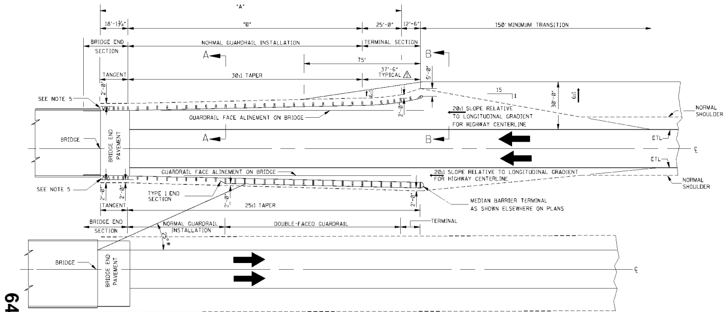
DIVIDED HIGHWAY WITH BARRIER INSIDE CLEAR ZONE OF OPPOSING TRAFFIC
