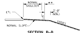
SECTION B-B
