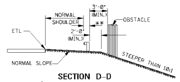
SECTION D-D FOR OBSTACLES 4' TO 17' FROM NORMAL SHOULDER
