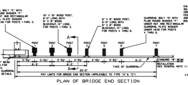
PLAN OF BRIDGE END SECTION * NOTE: UNLESS OTHERWISE SPECIFIED ON THE PLANS.
