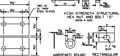
FASTENER DETAILS
