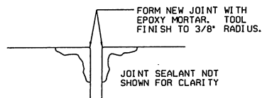
TYPICAL SECTION AT JOINT REPAIR SHOWING JOINT AFTER EPOXY MORTAR REPAIR
