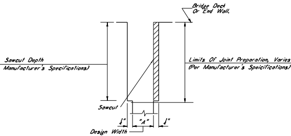
TYPICAL SECTION AT JOINT AFTER REMOVAL OF EXISTING SEAL Showing Limits Of Joint Preparation For Application Of New Joint Seal Materials
