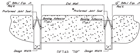
DETAIL "DP" Showing Sealed Joint After Saw Cut And Repair With Epoxy Mortar.
