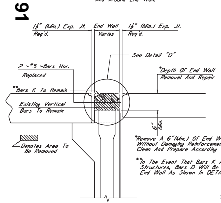
ELEVATION (SECTION A-A) Showing Details Of Removal Of Damaged End Wall.
