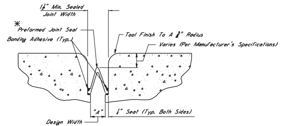
TYPICAL SECTION AT SAWCUT & SEALED JOINT Showing Repair With Epoxy Mortar And Preform Joint Seal
