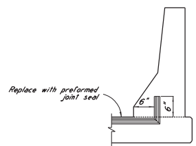
ELEVATION AT END OF SPAN
