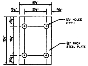
DETAIL OF PLATE "B"
