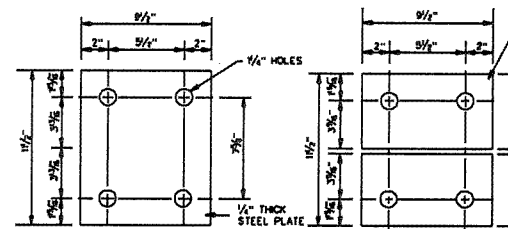
DETAIL OF PLATE "Z" CONCRETE BRIDGE RAIL TYPE "A" & "C"
