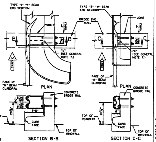
GUARDRAIL CONNECTION AT BRIDGE
