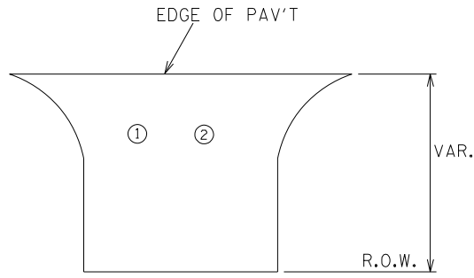
DETAIL FOR LOCAL ROAD TURNOUTS
