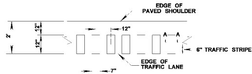
DETAIL "A"
