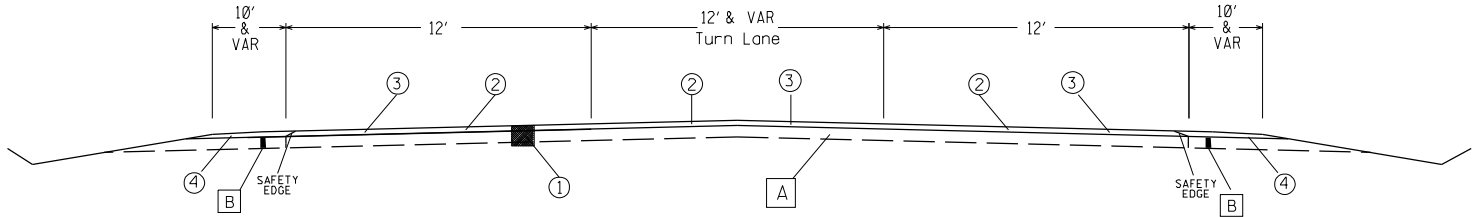
TYPICAL MILLING AND OVERLAY SECTION FOR 3-LANE SECTION WITHOUT CURB STA. 22+25 - 35+00
