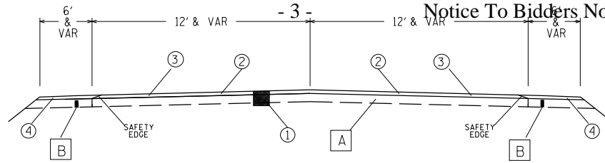
TYPICAL MILLING AND OVERLAY SECTION FOR 2-LANE SECTION STA. BOP 2+00 - 22+25
