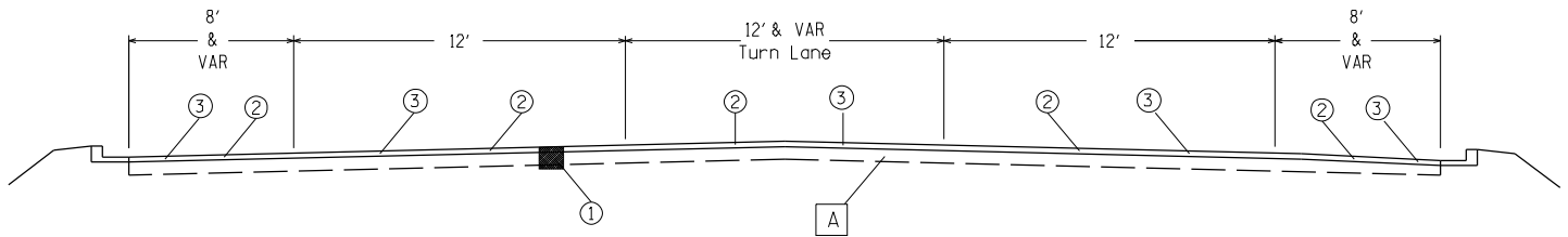
TYPICAL MILLING AND OVERLAY SECTION FOR 3-LANE SECTION WITH CURB STA. 35+00 - EOP 91+84
