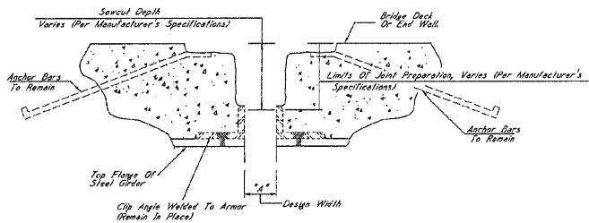
TYPICAL SECTION AT JOINT AFTER REMOVAL OF EXISTING MATERIAL
