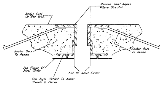
TYPICAL SECTION AT EXISTING JOINT
