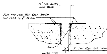
TYPICAL SECTION AT SAWCUT & JOINT REPAIR
