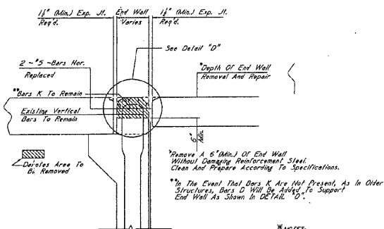
ELEVATION (SECTION A-A)
