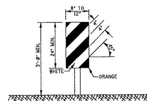
VERTICAL PANEL
