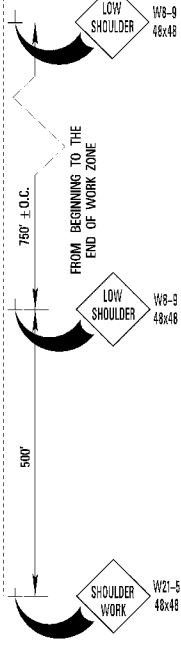
TYPICAL SHOULDER WORK #1
