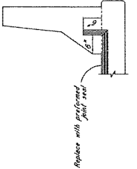
ELEVATION AT END OF SEAL Replace with preformed joint seal
