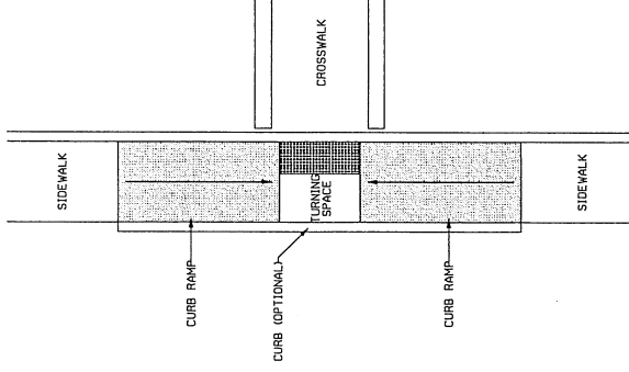
CURB RAMP CONFIGURATION: TYPE H
