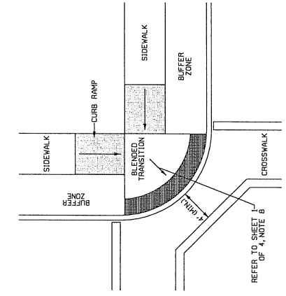
CURB RAMP CONFIGURATION: TYPE J NOT RECOMMENDED
