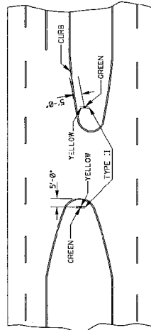
TYPICAL DELINEATION AT A CURBED CROSSOVER WITH A MEDIAN WIDTH OF 40'-0" OR LESS
