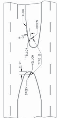
TYPICAL DELINEATION AT A CURBED CROSSOVER WITH A MEDIAN WIDTH OF 40'-0" OR LESS
