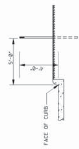
DELINEATOR MOUNTING ON CURBED CROSSOVER
