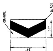
CHEVRON SIGN DETAIL
