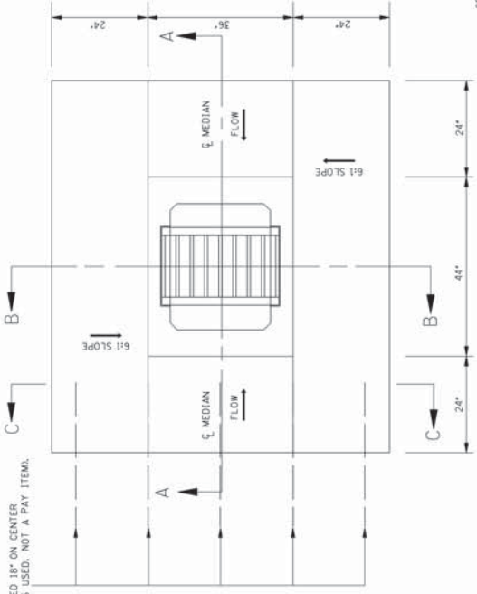
PLAN OF INLET & PAVED APRON
