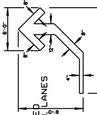
DETAIL OF TEMPORARY TURN ARROW
