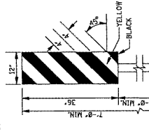
TYPE 3 OBJECT MARKER (OM-3R)
