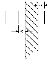
DETAIL B LATERAL PLACEMENT OF PAVEMENT MARKERS
