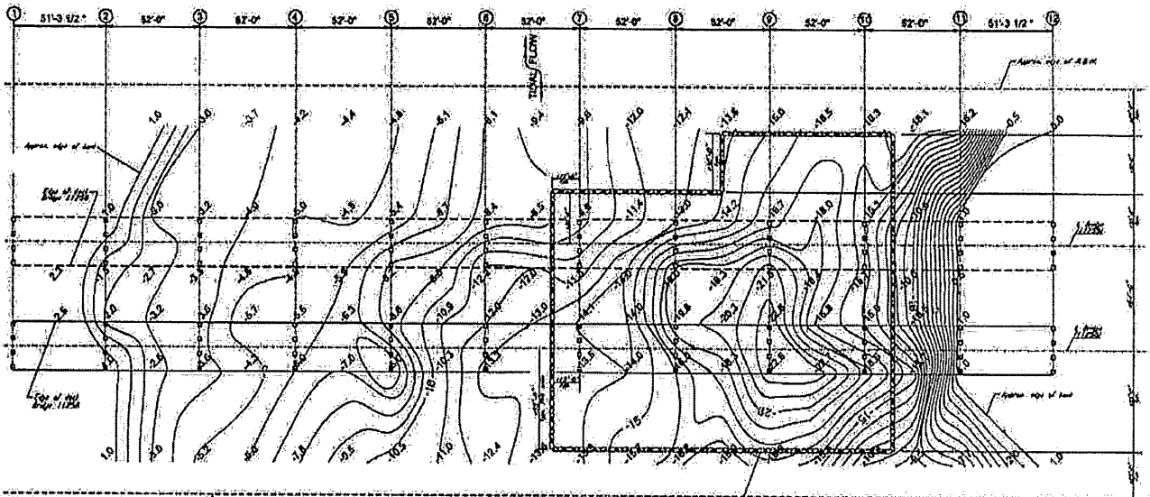
PLAN VIEW RIPRAP PLACEMENT
