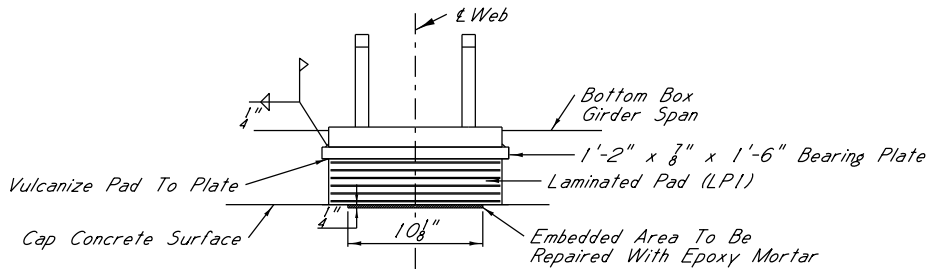
Showing elevation of bearing assembly at Bents 1 and 5
