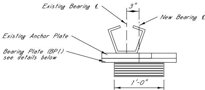
Showing side elevation of bearing assembly at Bents 1 and 5
