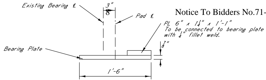
Showing side elevation of built up bearing plate (BPI)
