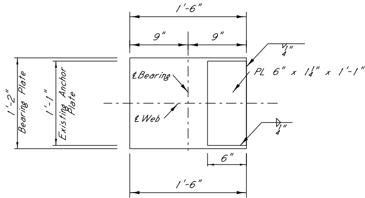
Showing side elevation of built up bearing plate (BPI)
