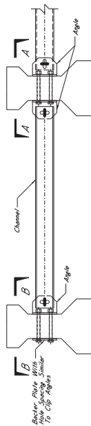
TEMPORARY STEEL BRACING DETAILS AASHTO Type-1A, 2, 3, 4, & Type-1A, 2 Beams
