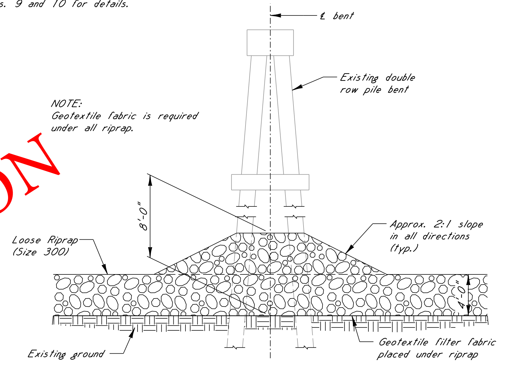
RIPRAP PLACEMENT AT BENT
