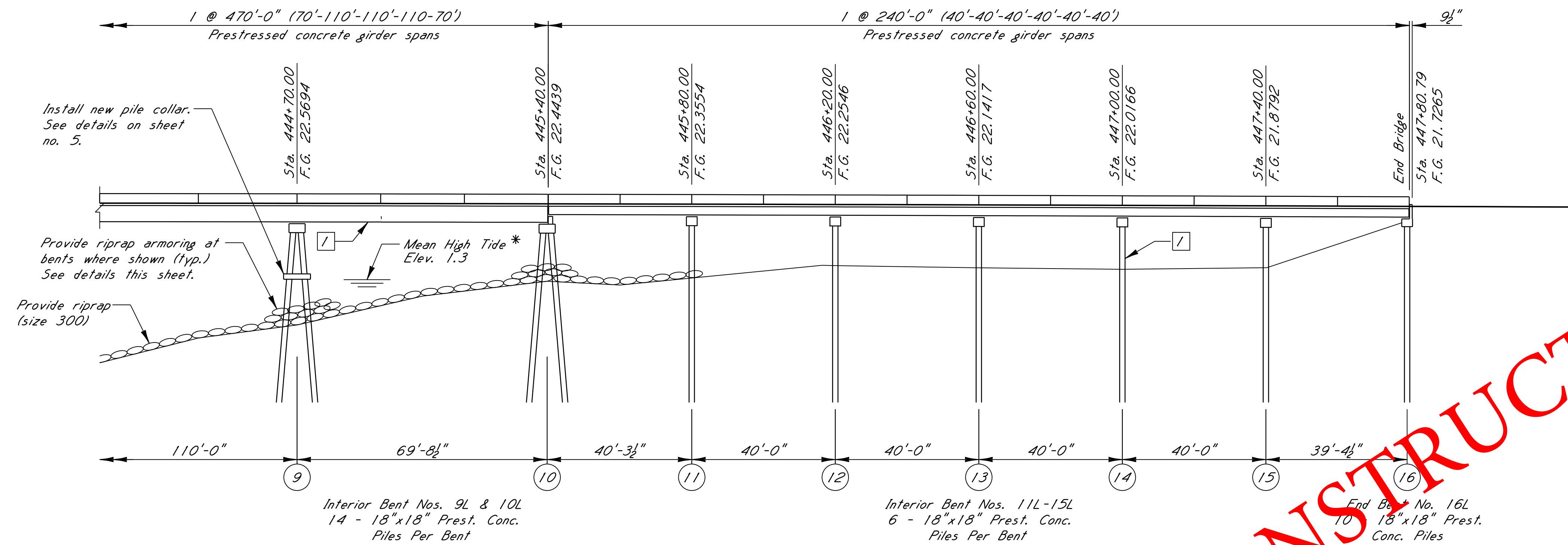
LEFT LANE ELEVATION WITH PROFILE ALONG & BRIDGE Scale: 1" = 20'-0"
