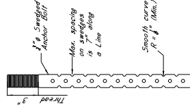
SWEGED ANCHOR BOLT DETAIL
