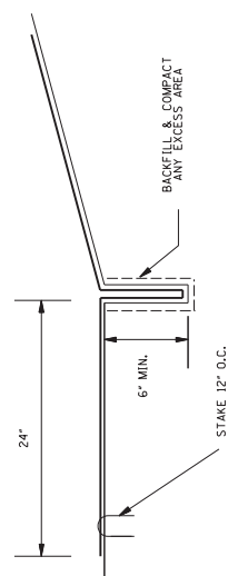
DETAIL OF BOTTOM TRENCH
