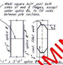
PILE SPICE DETAIL HP14x117 Steel Piles
