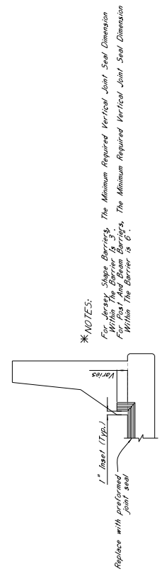
ELEVATION AT END OF SPAN
