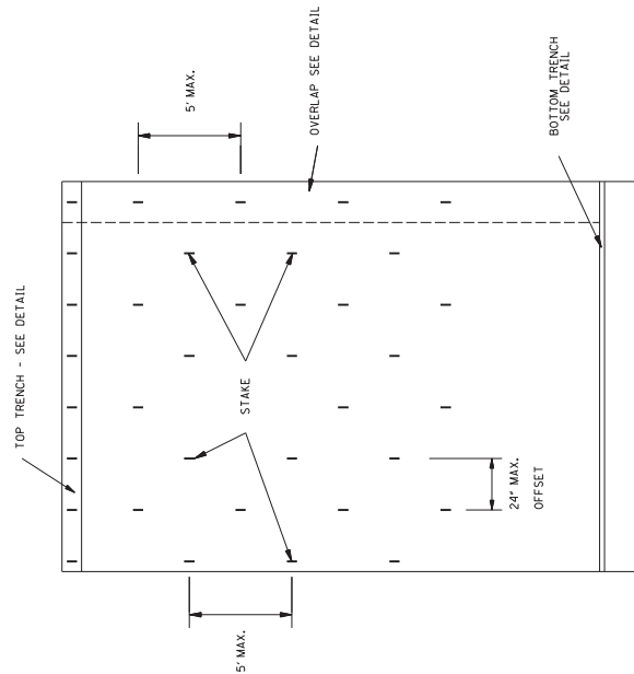
DETAIL OF EROSION CONTROL BLANKET
