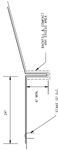
DETAIL OF BOTTOM TRENCH
