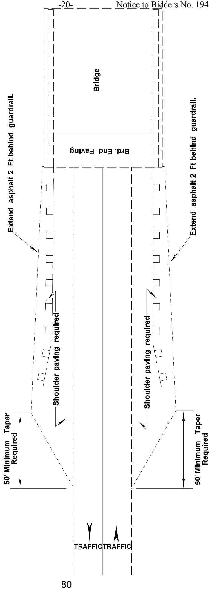
TYPICAL DETAIL OF ADDITIONAL SHOULDER PAVING REQUIRED AT GUARDRAIL LOCATIONS
