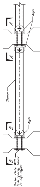
TEMPORARY STEEL BRACING DETAILS AASHTO Type-1A, 2, 3, 4, 5, & Type-1A, 2 Beams
