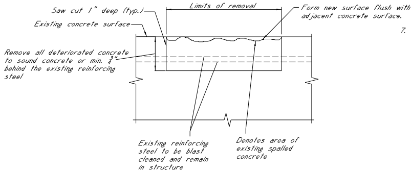
ELEVATION OF SPALL REPAIR DETAILS
