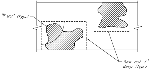
PLAN OF SPALL REPAIR DETAILS
