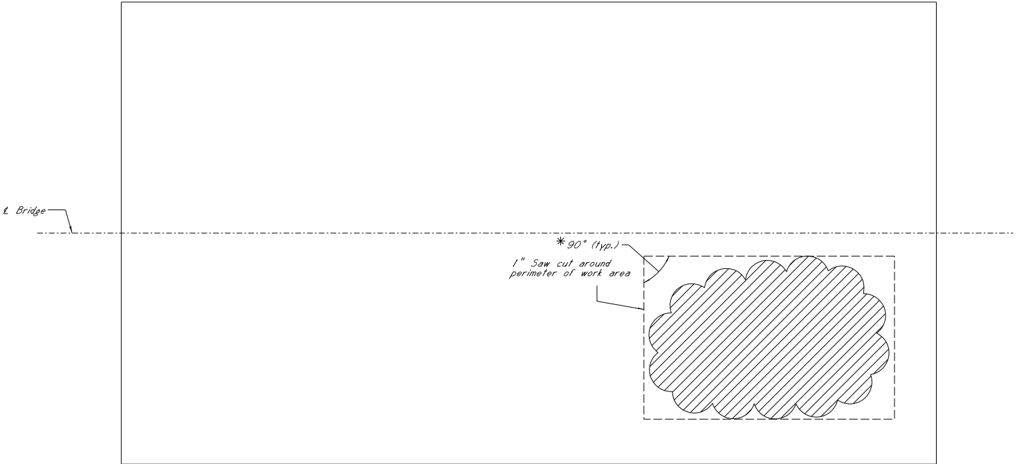
SPALL REPAIR LOCATION Showing approximate location of repair area
